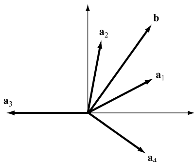
Fig. 3.1 Constraint representation in requirements space
