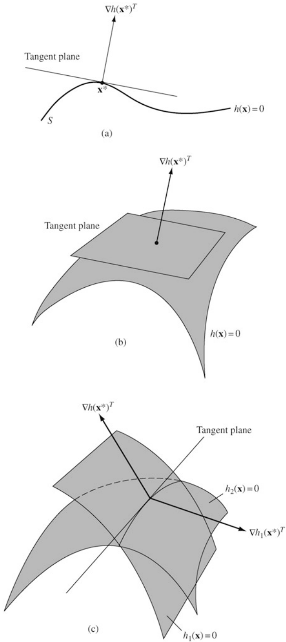
Fig. 11.2 Three examples of tangent planes (translated to x^* )
