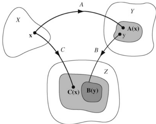
Fig. 7.7 Composition of mappings
