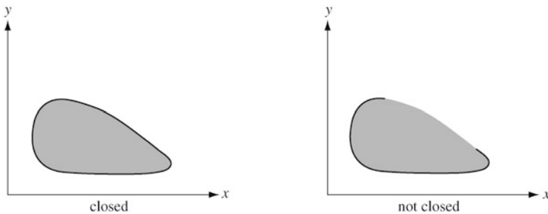
Fig. 7.6 Graphs of mappings
