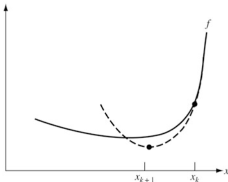
Fig. 8.5 Newton's method for minimization
