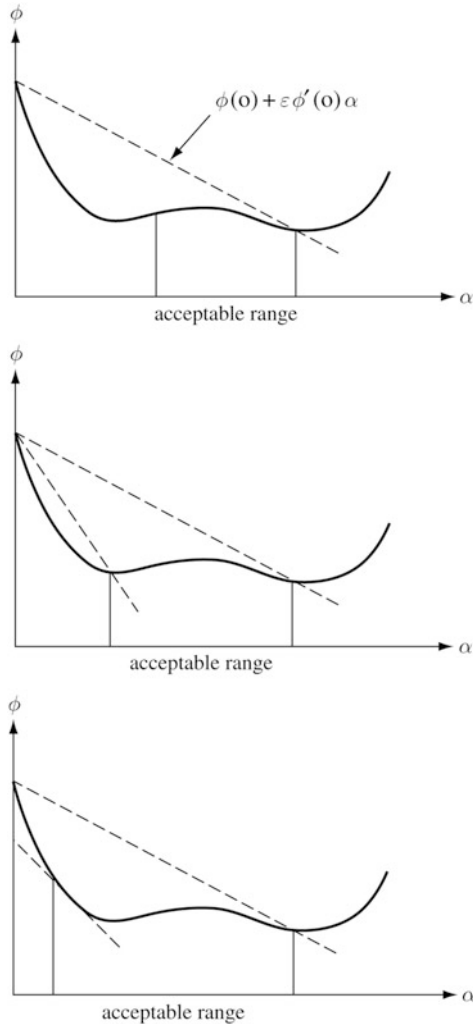
Fig. 8.8 Stopping rules. (a) Armijo rule. (b) Golden test. (c) Wolfe test
