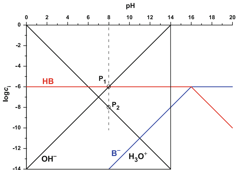
Fig. 46 pH-log c i diagram of an aqueous solution prepared by dissolving 10^{-6} mol of sodium ethanolate in water so that 1 l of solution results. The range \text{pH} > 14 is shown for didactic reasons only. Normally it is not shown
