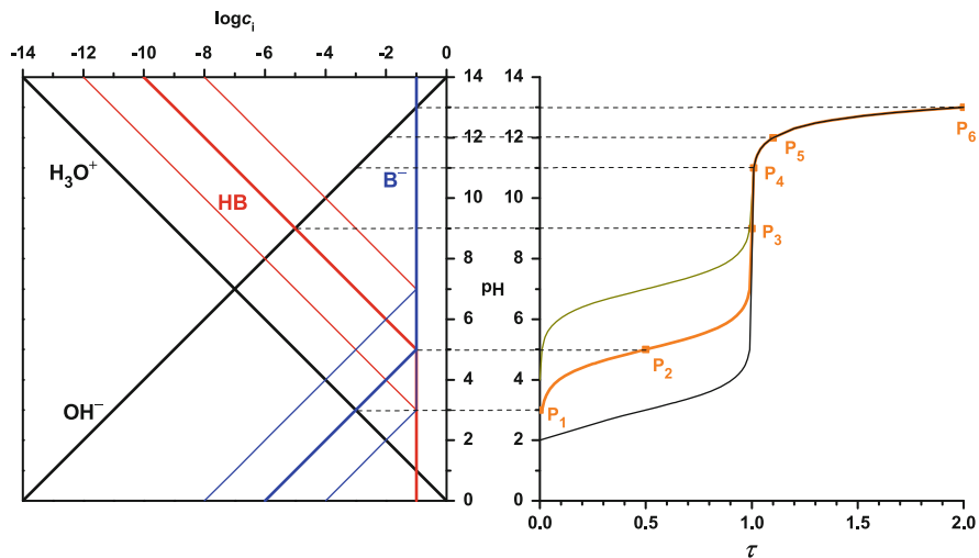
Fig. 79 Titration diagrams of three acids ( \log C_{acid}^O = -1 ) with pK_a = 3 (black line); pK_a = 5 (orange line) and pK_a = 7 (olive line) with sodium hydroxide solution. The distinctive points are given only for pK_a = 5
