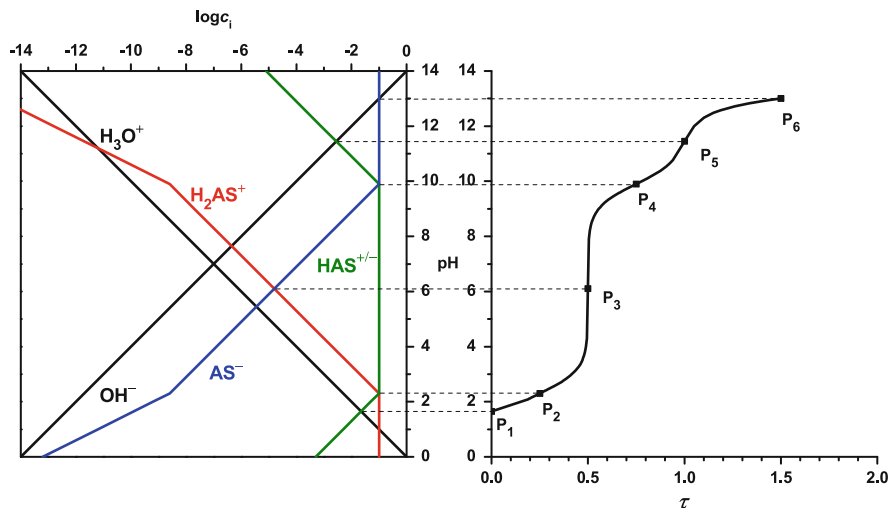
Fig. 82 Titration diagram of alanine ( \log C_{\text{alanine}}^{\circ} = -1 , \text{p}K_{\text{a}1} = 2.3 , \text{p}K_{\text{a}2} = 9.9 ) with sodium hydroxide
