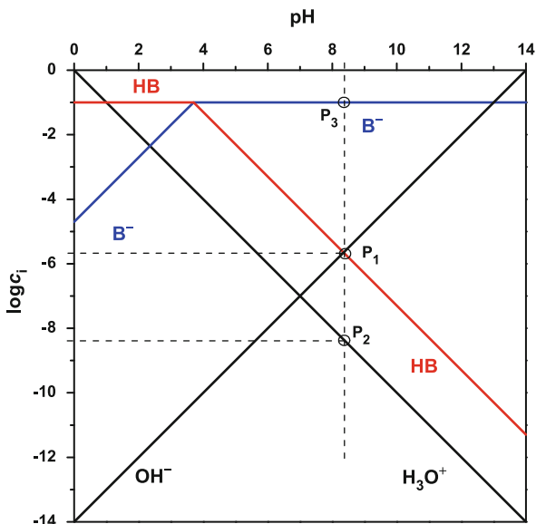
Fig. 39 pH- \log c_i diagram of sodium formate solution at C_{\text{HB}}^{\circ} = 10^{-1} \text{ mol L}^{-1} (Formic acid: \text{p}K_{\text{a}} = 3.75 )
