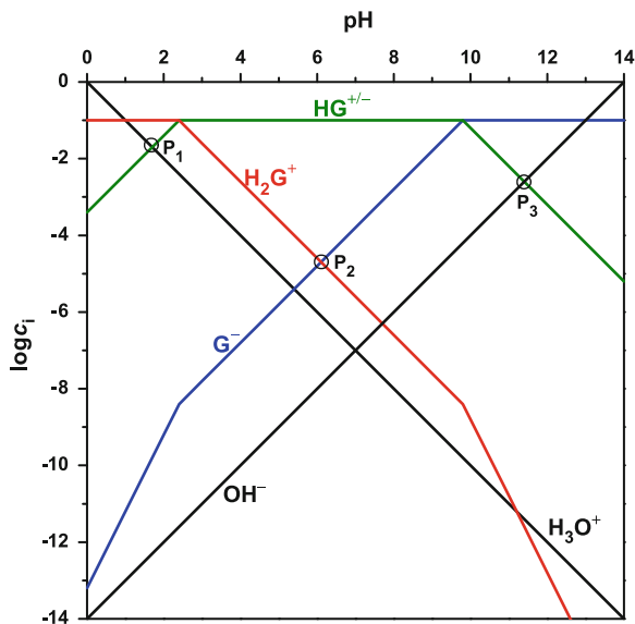
Fig. 68 pH-log i diagram of glycine at an overall concentration of 0.1 mol L -1
