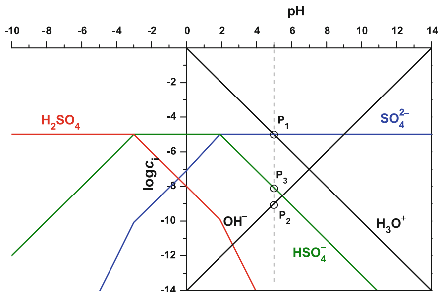
Fig. 49 pH- \log c_i diagram of sulfuric acid at 10^{-5} mol L -1 . The range pH < 0 is shown for didactic reasons only. Normally it is not shown
