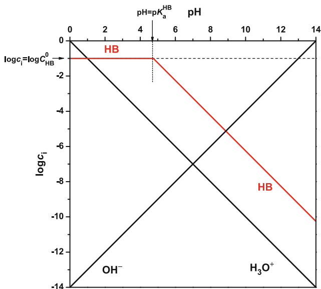
Fig. 13 Plotting the two asymptotes of HB with Eq. (33) for \text{pH} < \text{p}K_a and Eq. (34) for \text{pH} > \text{p}K_a . Example: acetic acid with C_{\text{HB}}^0 = 0.1 \text{ mol L}^{-1} and \text{p}K_a = 4.75
