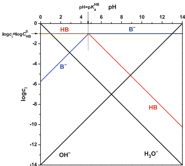
Fig. 14 Plotting the two asymptotes of \text{B}^- with Eq. (35) for \text{pH} < \text{p}K_a and Eq. (36) for \text{pH} > \text{p}K_a . Example: acetic acid with C_{\text{HB}}^0 = 0.1 \text{ mol L}^{-1} and \text{p}K_a = 4.75
