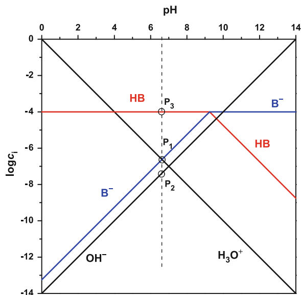
Fig. 42 pH-log c_i diagram of an ammonium chloride solution at C_{\text{HB}}^{\circ} = 10^{-4} mol L ^{-1} (ammonium: pK_a = 9.25 )
