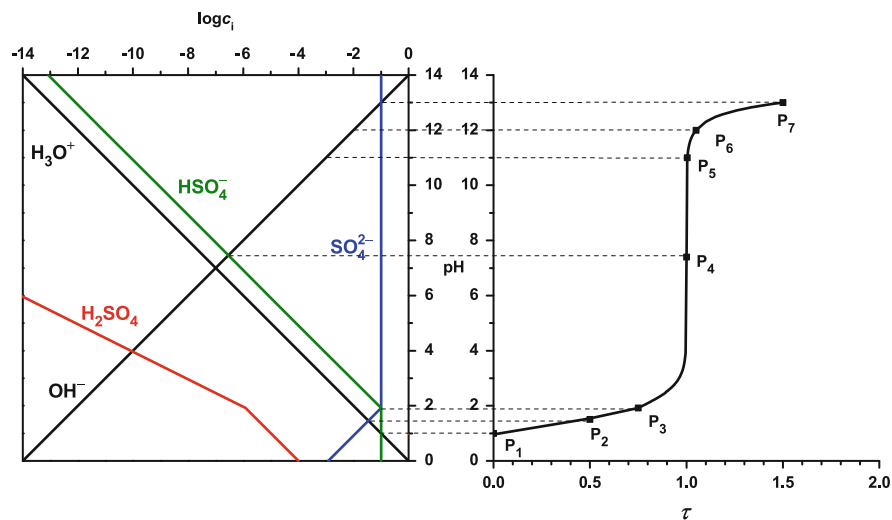
Fig. 81 Titration diagram of sulfuric acid ( \log C_{\text{sulfuric acid}}^{\text{O}} = -1 ), \text{p}K_{\text{a}1} = -3 , \text{p}K_{\text{a}2} = 1.99 with sodium hydroxide
