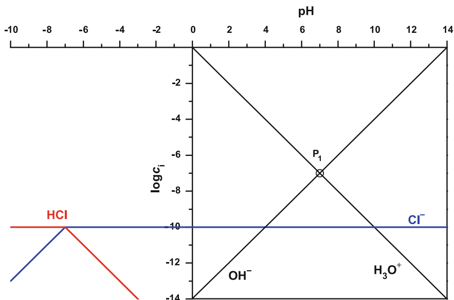
Fig. 34 pH- \log c_i diagram of a hydrochloric acid ( pK_a = -7 ) at 10^{-10} mol L ^{-1} concentration. The range for pH < 0 is only shown for didactic reasons. Normally this is not done
