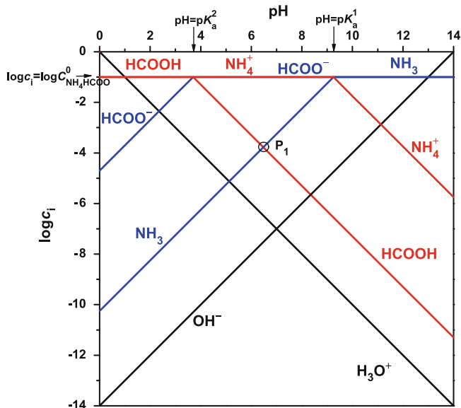
Fig. 56 pH-log i c i diagram of a solution containing 0.1 mol L -1 ammonium formate
