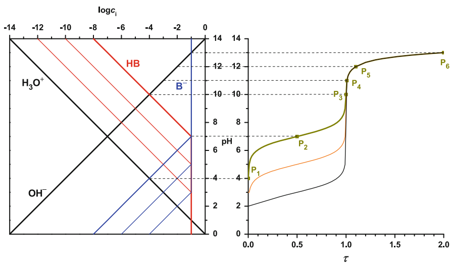
Fig. 80 Titration diagrams of three acids ( \log C_{acid}^O = -1 ) with pK_a = 3 (black line); pK_a = 5 (orange line) and pK_a = 7 (olive line) with sodium hydroxide solution. The distinctive points are given only for pK_a = 7
