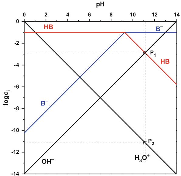
Fig. 43 pH-log c i diagram of an ammonia solution, C_{\text{ammonia}}^{\circ} = 10^{-1} \text{ mol L}^{-1} (Ammonium: \text{p}K_{\text{a}} = 9.25 )
