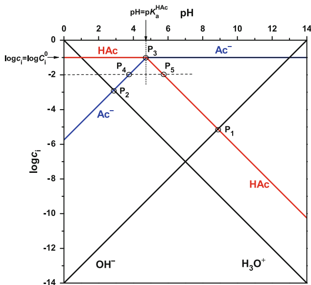
Fig. 61 pH-log i diagram of the corresponding acid–base pair acetic acid/acetate ions \log C_i^0 = -1.00 , \text{p}K_a = 4.75
