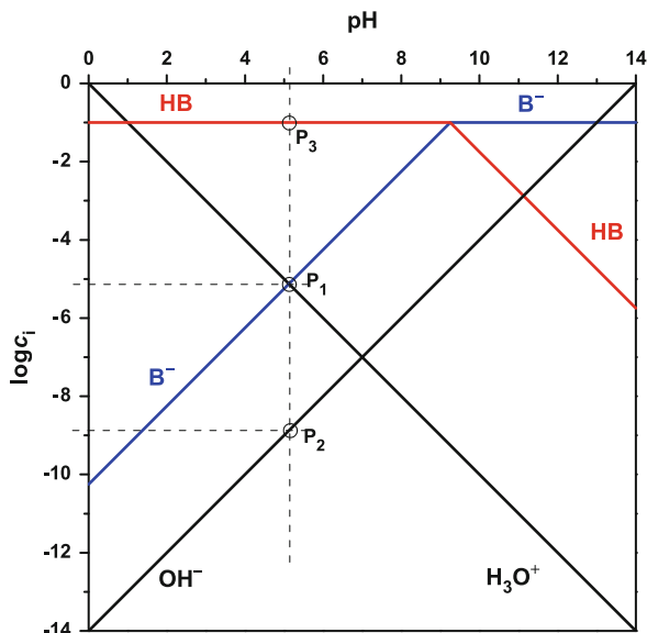
Fig. 41 pH-log c_i diagram of an ammonium chloride solution at C_{\text{HB}}^{\circ} = 10^{-1} mol L ^{-1} (ammonium: pK_a = 9.25 )
