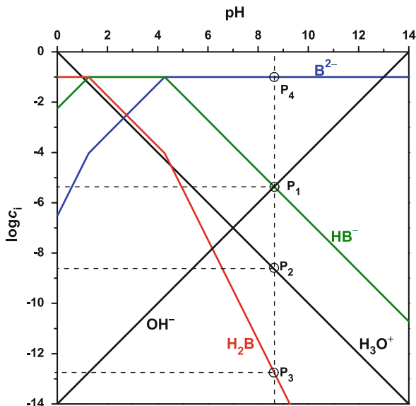
Fig. 55 pH-log c i diagram of a solution containing 0.1 mol L -1 of sodium oxalate (oxalate: pK b1 = 9.73 and pK b2 = 12.73)
