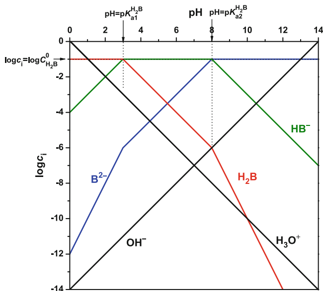
Fig. 19 Plotting the three lines of B^{2-} in the ranges \text{pH} < \text{p}K_{a1} , \text{p}K_{a1} < \text{pH} < \text{p}K_{a2} and \text{pH} > \text{p}K_{a2} . Example: acid with \log C_{H_2B}^0 = -1 , \text{p}K_{a1} = 3 and \text{p}K_{a2} = 8
