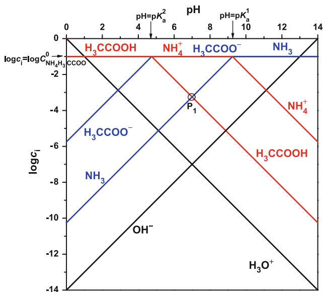
Fig. 57 pH-log i c i diagram of a solution containing 0.1 mol L -1 ammonium acetate
