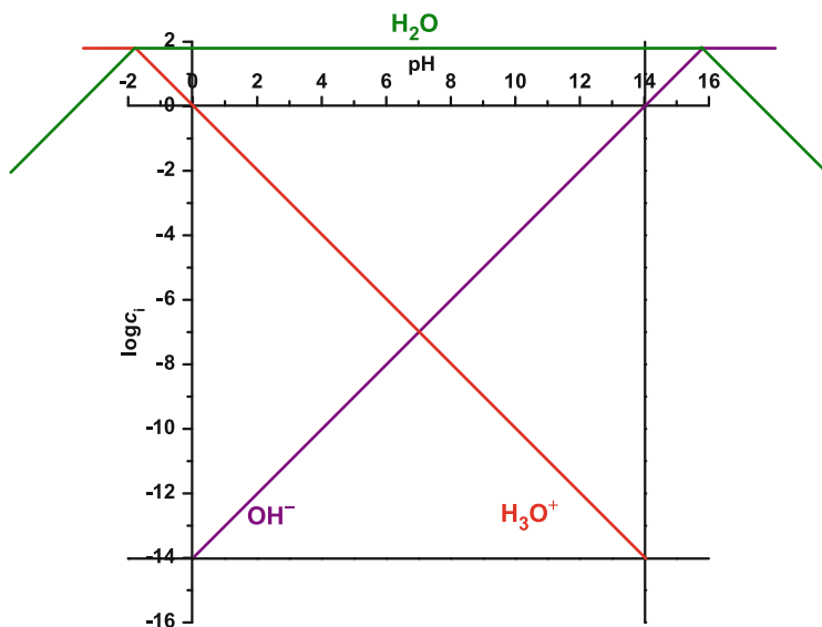
Fig. 60 pH- \log c_i diagram of water with \log C_{\text{H}_2\text{O}}^{\circ} = 1.74 and the two not entirely correct values \text{p}K_{\text{a}}(\text{H}_3\text{O}^+) = -1.74 and \text{p}K_{\text{a}}(\text{H}_2\text{O}) = 15.74
