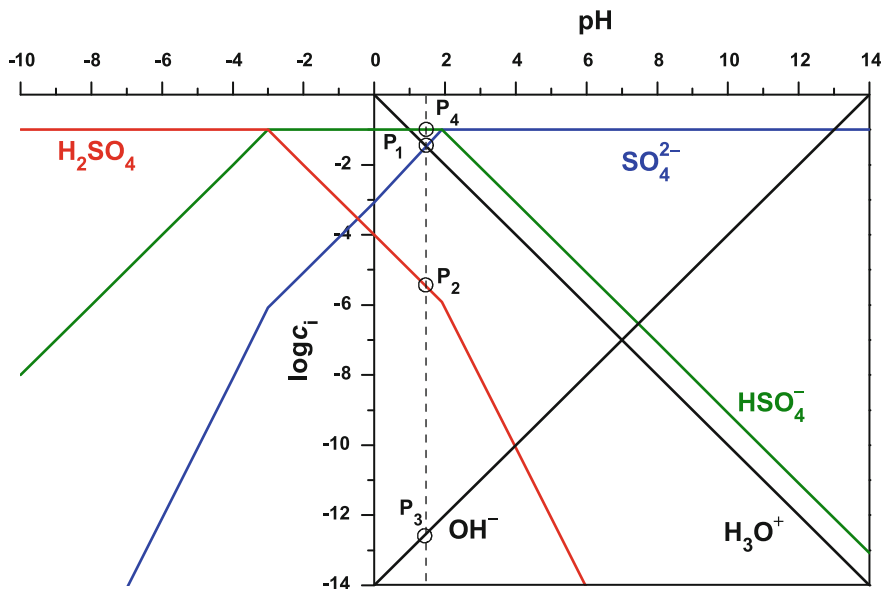
Fig. 52 pH-log c i diagram of a NaHSO 4 solution at 10 -1 mol L -1 (pK a2 = 1.99 and pK b2 = 17). The range pH < 0 is shown for didactic reasons only. Normally it is not shown
